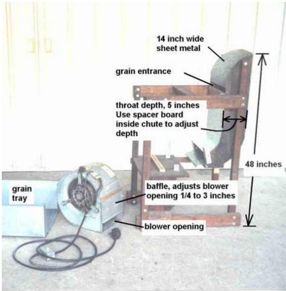
Fig. 2 Winnower, disassembled
