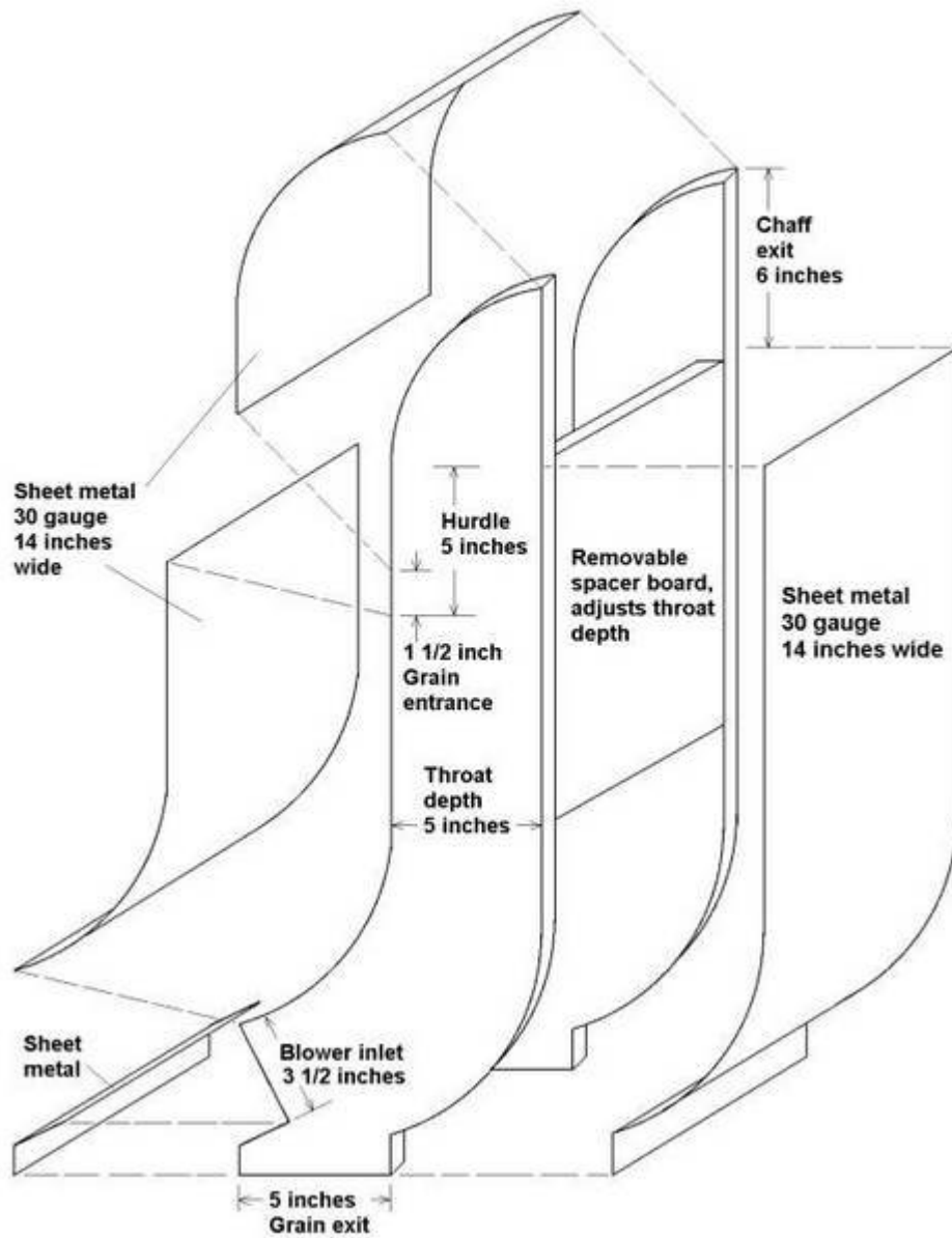
Figure 3. Exploded view of winnower chute
