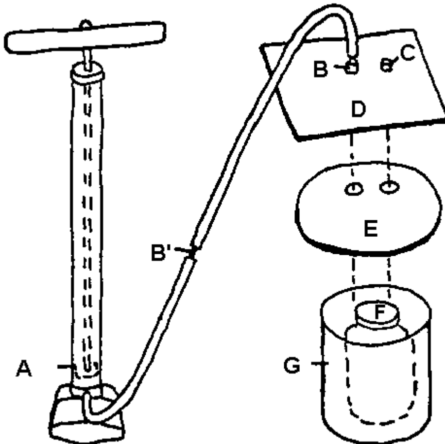
Figure 1. The vacuum packing system for seed storage.
